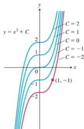
FIGURE 4.52 The curves y = x^3 + C fill the coordinate plane without overlapping. In Example 2, we identify the curve y = x^3 - 2 as the one that passes through the given point (1, -1) .
