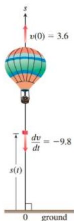
FIGURE 4.53 A package dropped from a rising hot-air balloon (Example 5).
